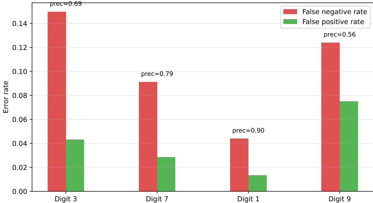
MNIST: filter error rates ( N_S = 200 )
