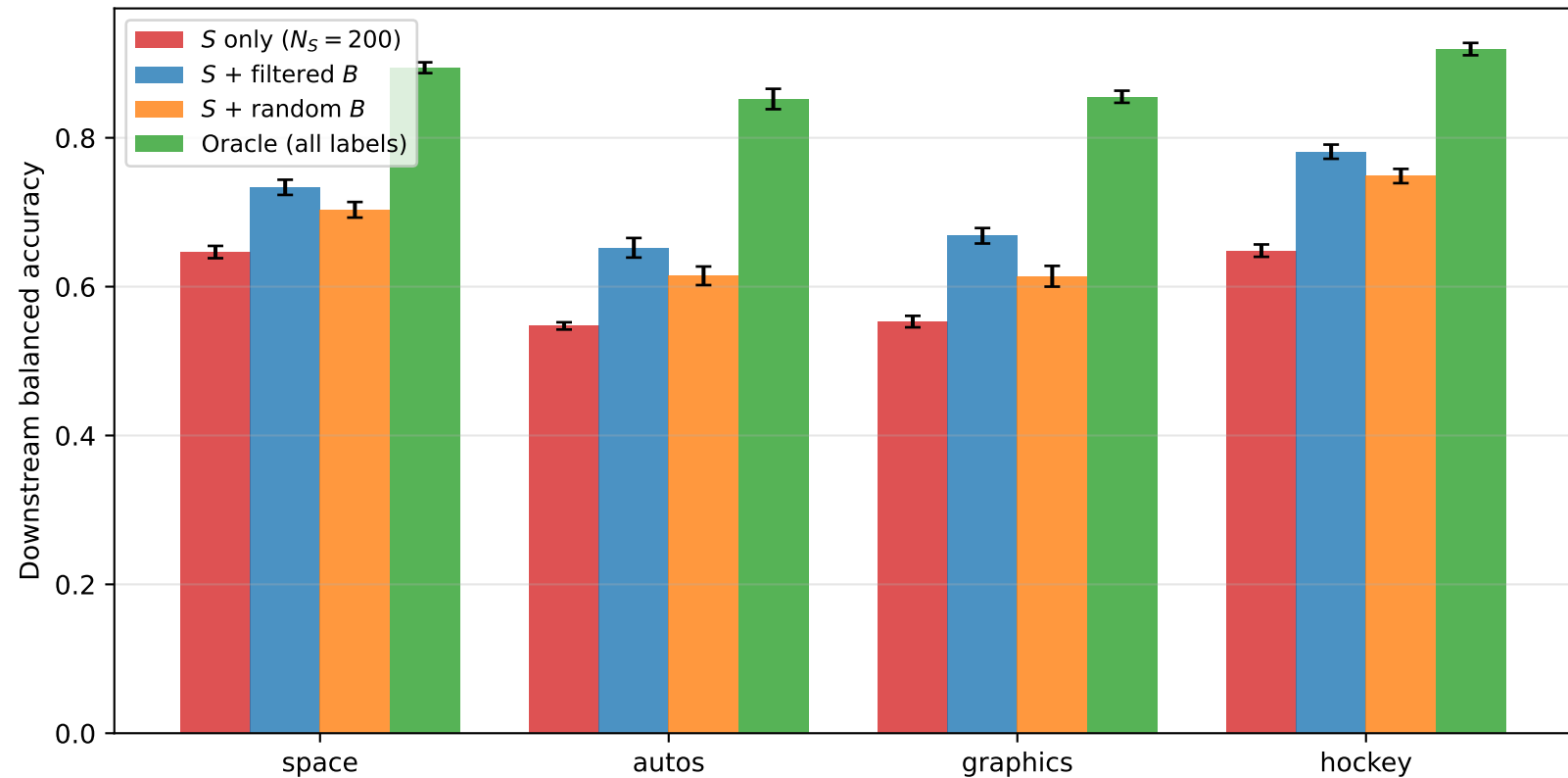
20 Newsgroups: filtering improves downstream classification
