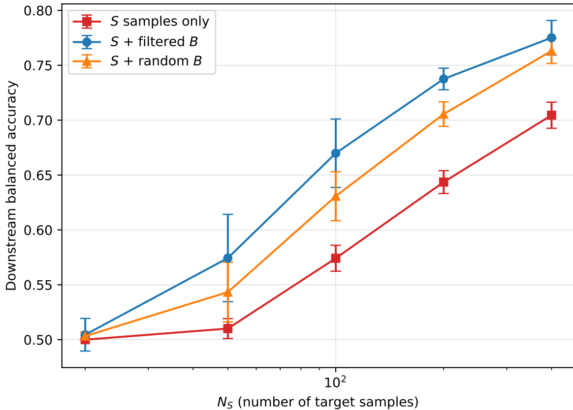
20 Newsgroups (sci.space): accuracy vs N_S
