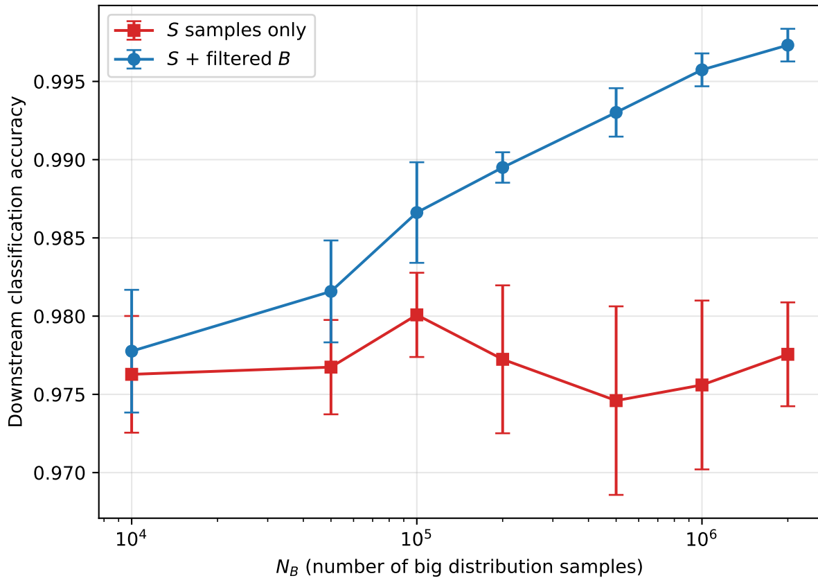
Downstream accuracy vs N_B ( N_S = 1000 , p = 0.01 )
