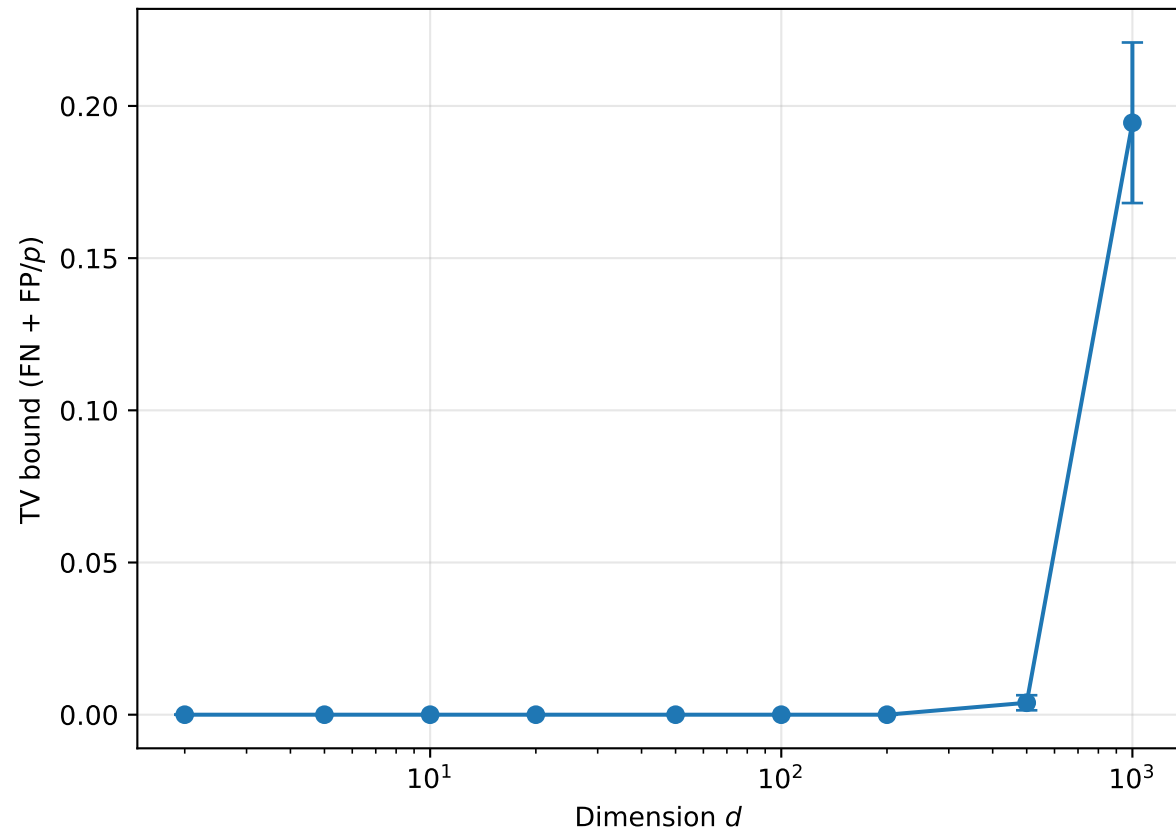
TV bound vs dimension d ( N_S = 1000 , N_B = 500,000 , p = 0.01 )
