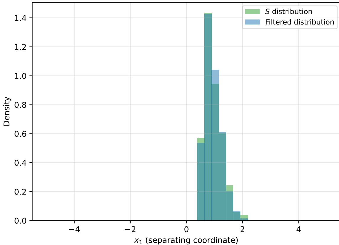
Distribution comparison (TV \approx 0.111 )
