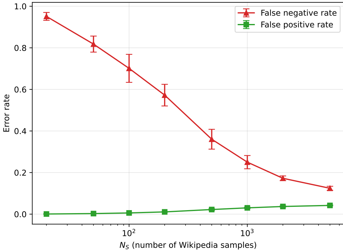
Wikipedia vs C4 (bge, 768d): filter errors vs N_S
