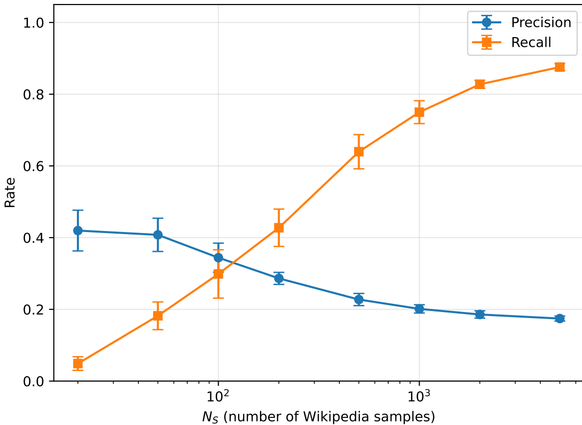
Wikipedia vs C4 (bge, 768d): precision/recall vs N_S
