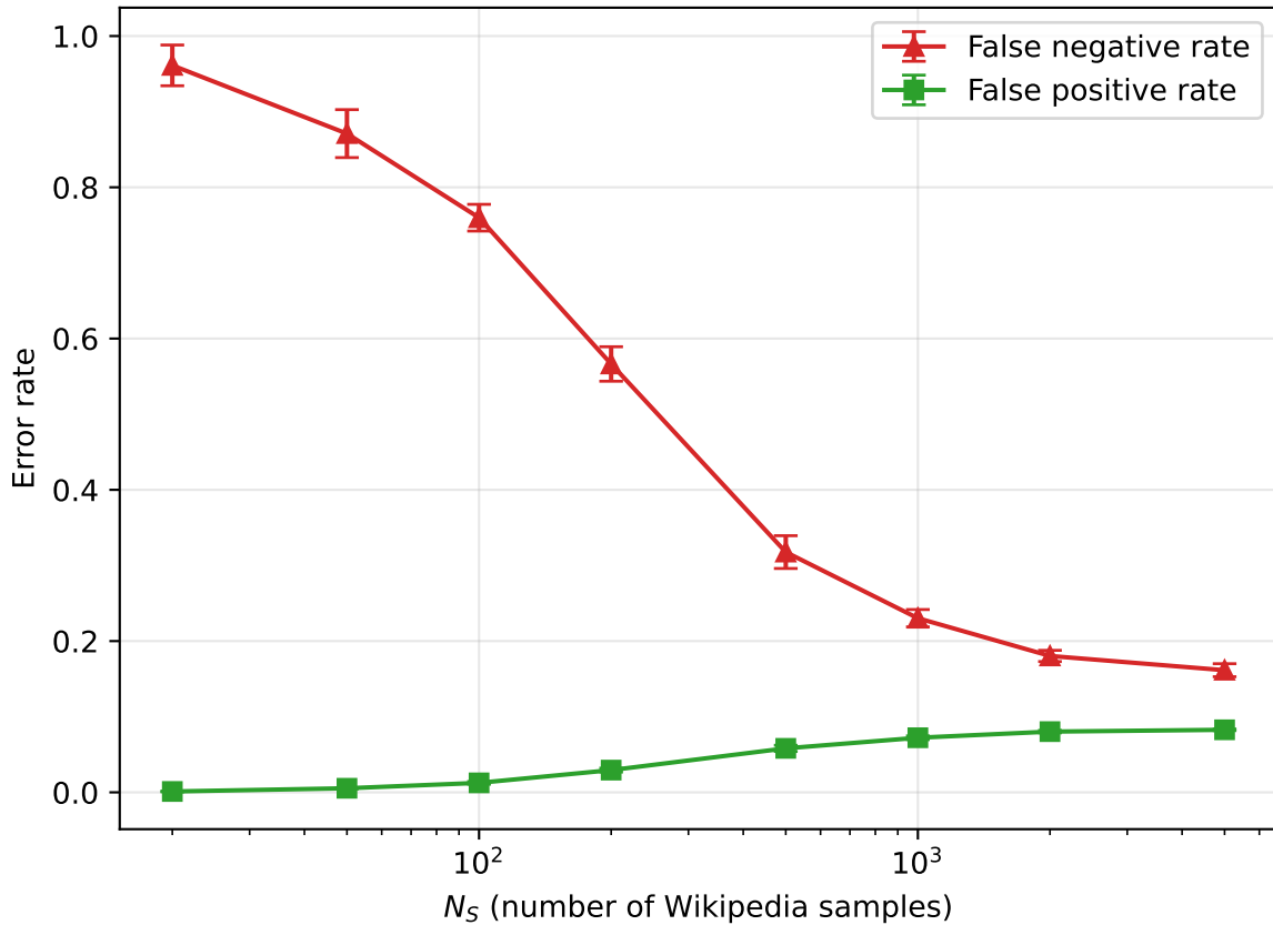
Wikipedia vs C4 (minilm, 384d): filter errors vs N_S
