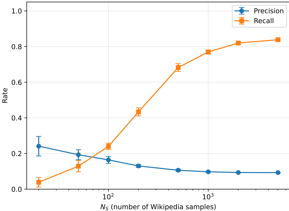
Wikipedia vs C4 (minilm, 384d): precision/recall vs N_S
