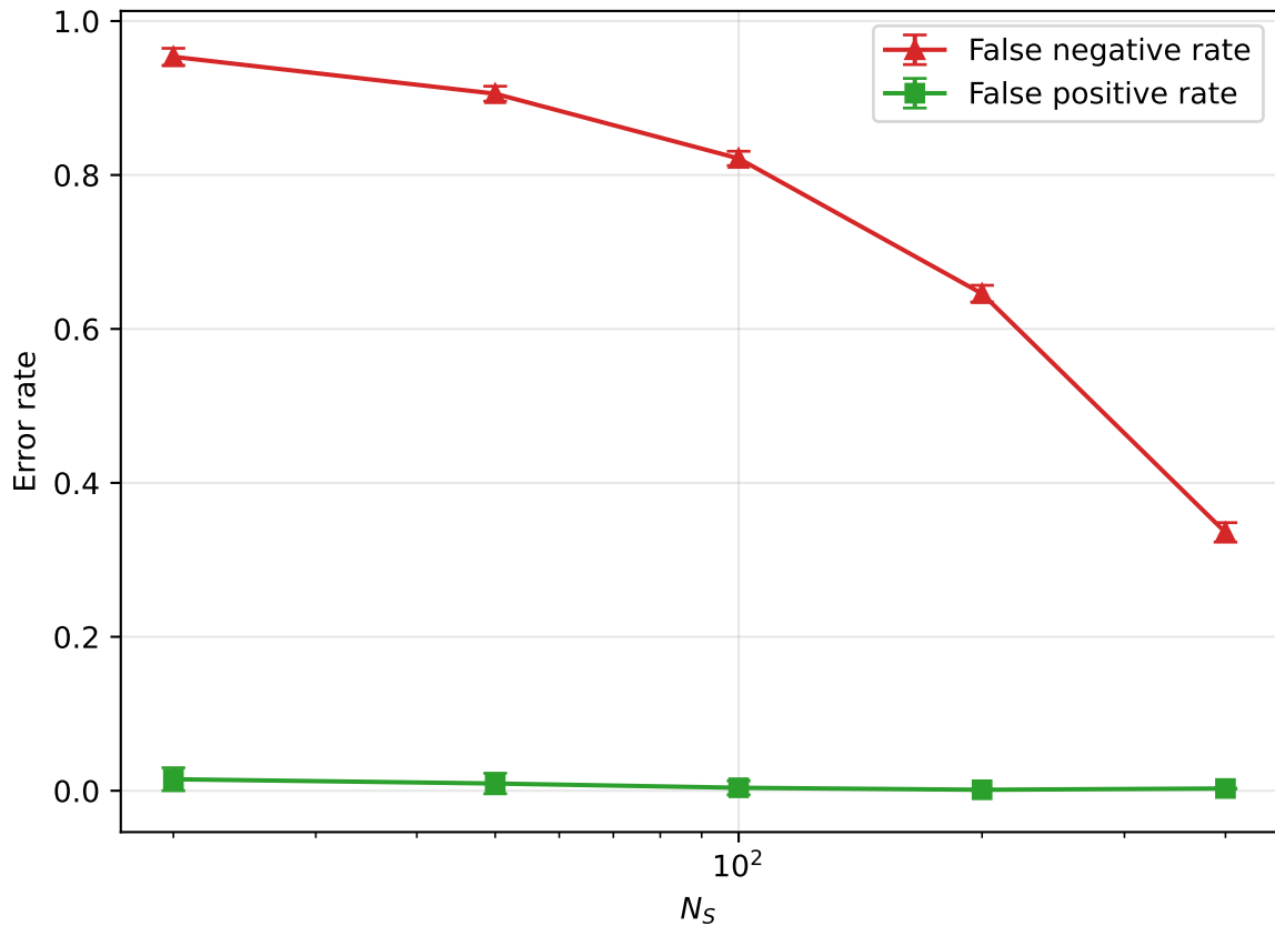
20 Newsgroups (sci.space): filter errors vs N_S
