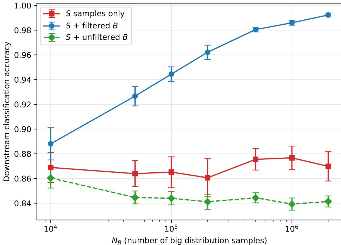
Downstream accuracy vs N_B ( N_S = 200 , p = 0.01 )
