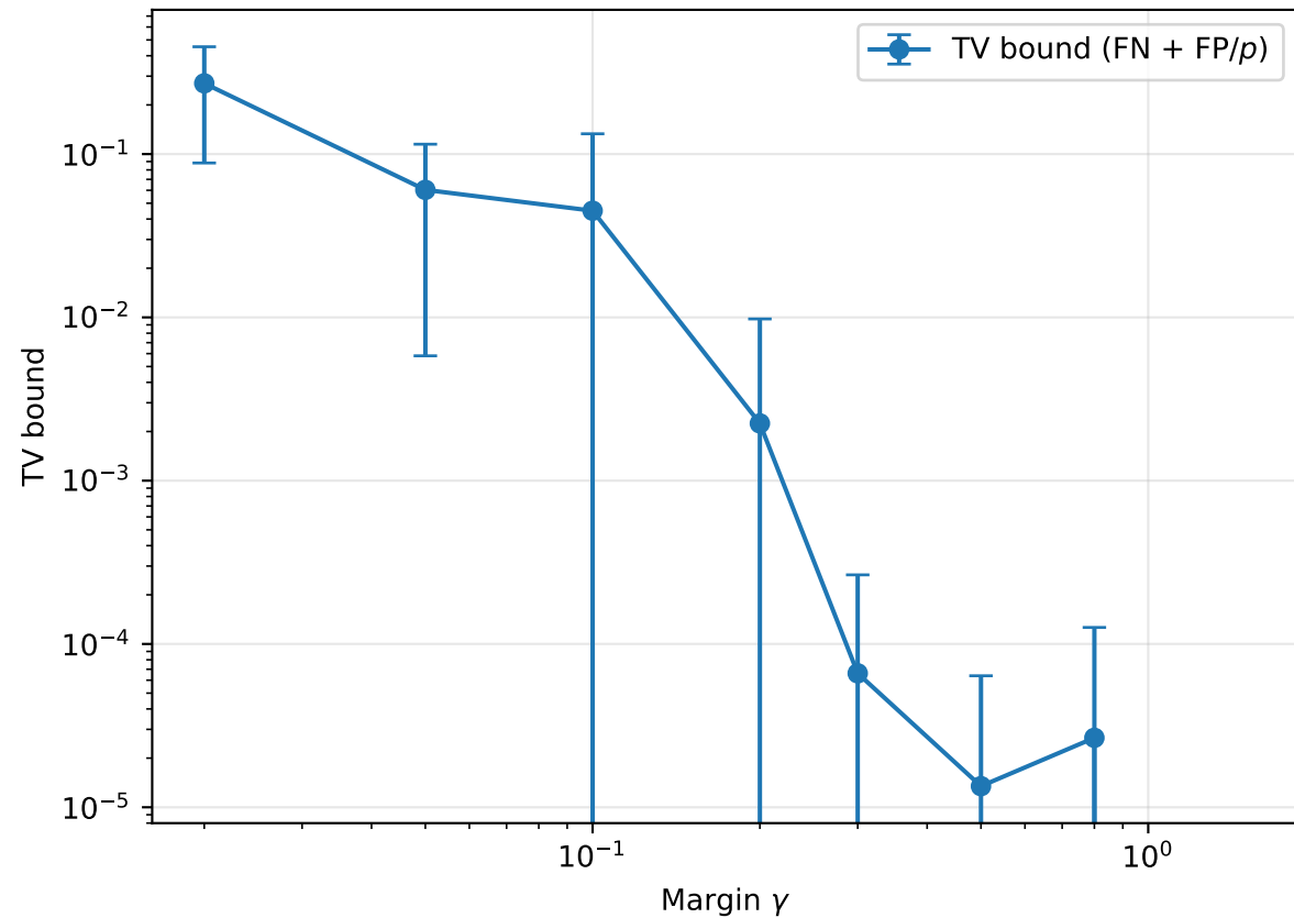
TV bound vs margin \gamma ( N_S = 30 , p = 0.01 , R = 3.0 )
