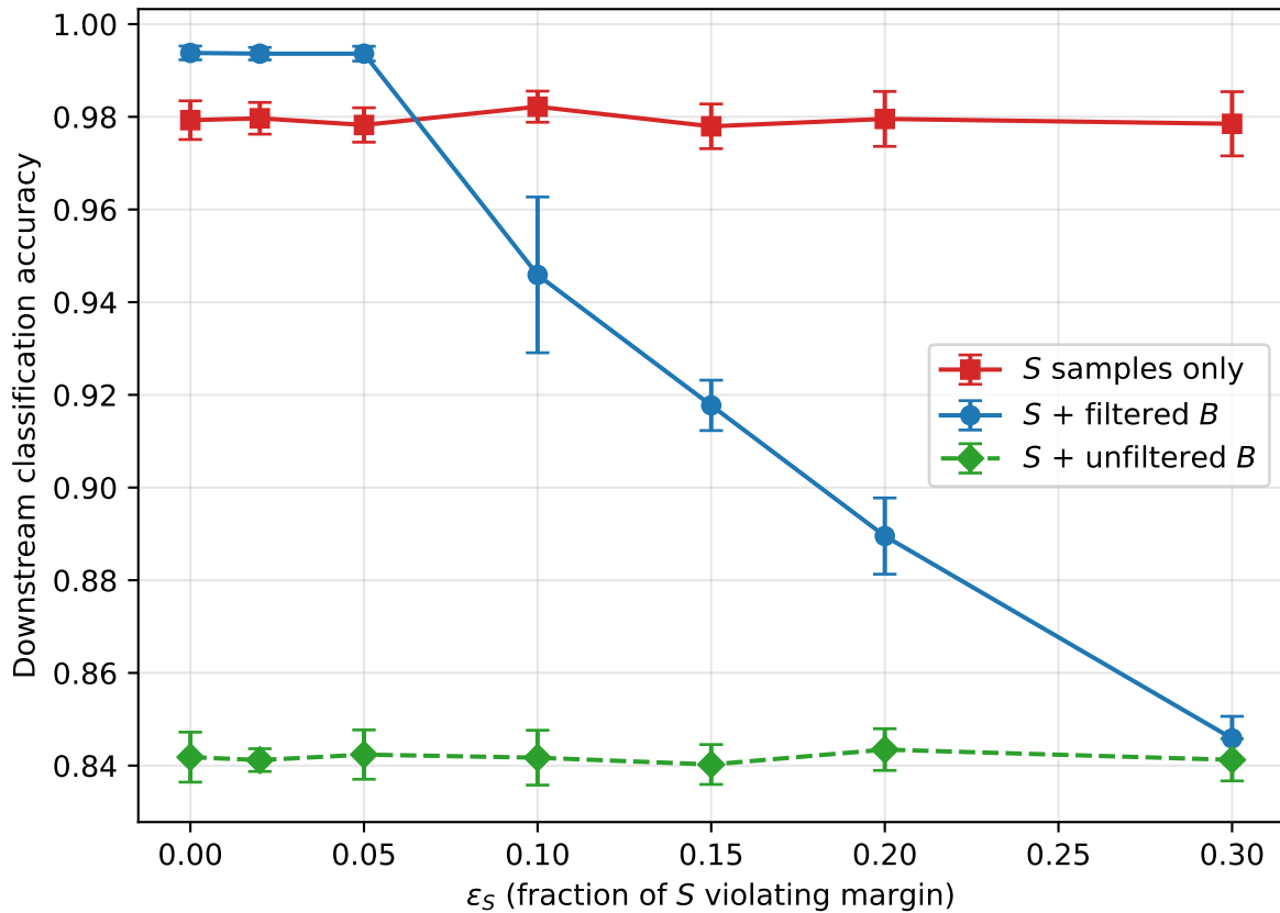
Downstream accuracy vs \varepsilon_S
