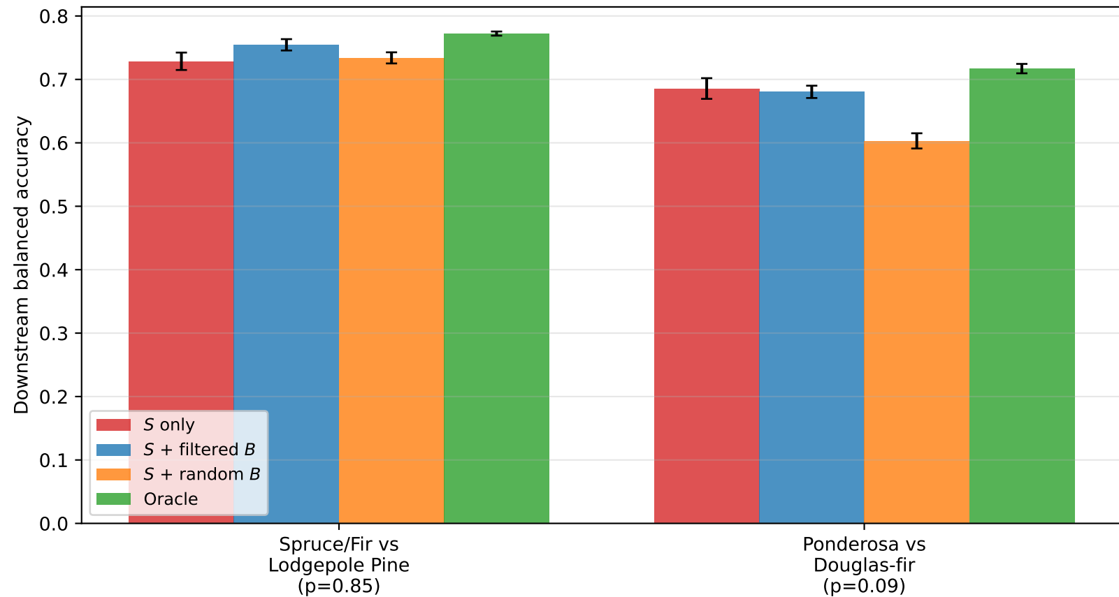
Covertypes: filtering improves within-S classification ( N_S = 200 )
