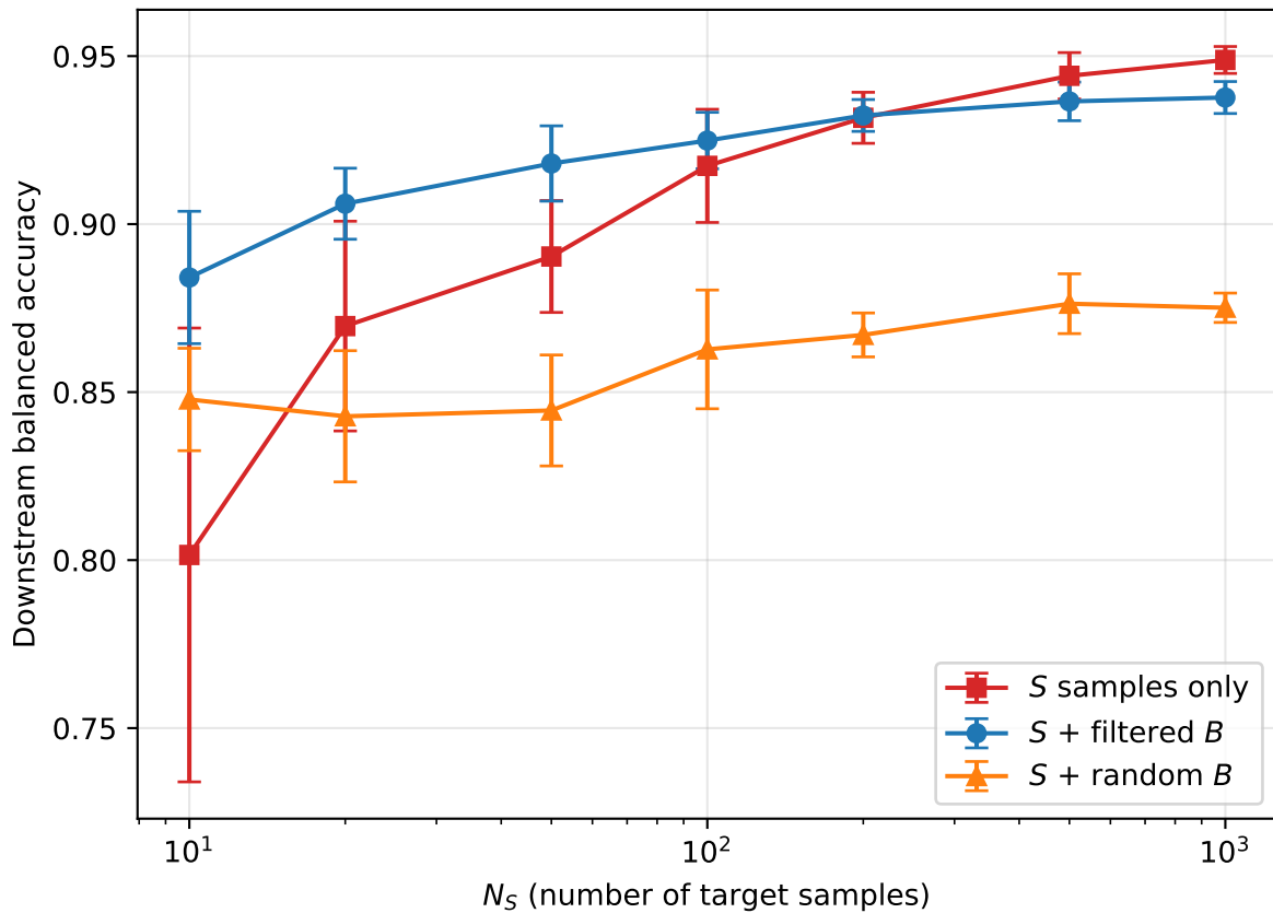
MNIST (7 vs 9): accuracy vs N_S
