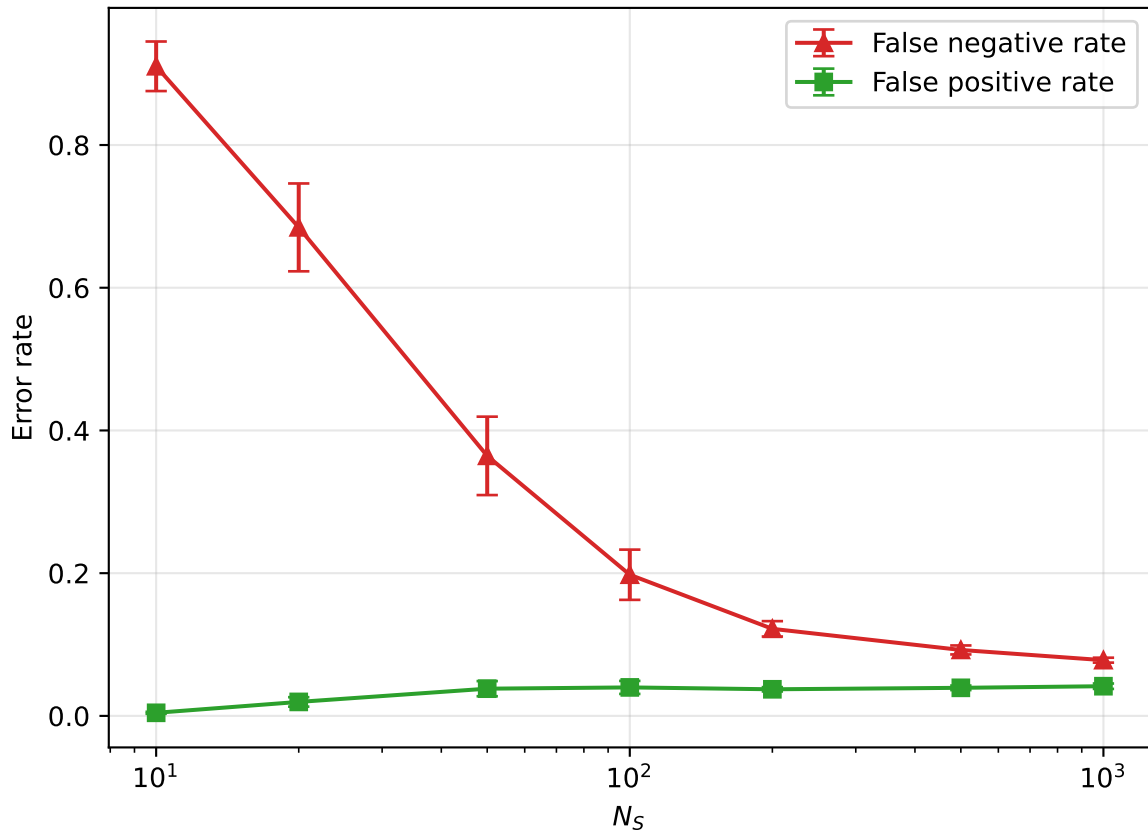
MNIST (7 vs 9): filter errors vs N_S
