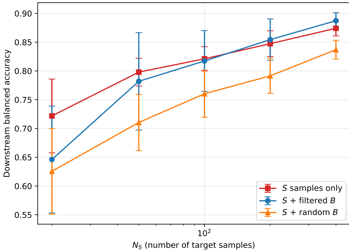
20 Newsgroups (sci.crypt vs sci.electronics): accuracy vs N_S
