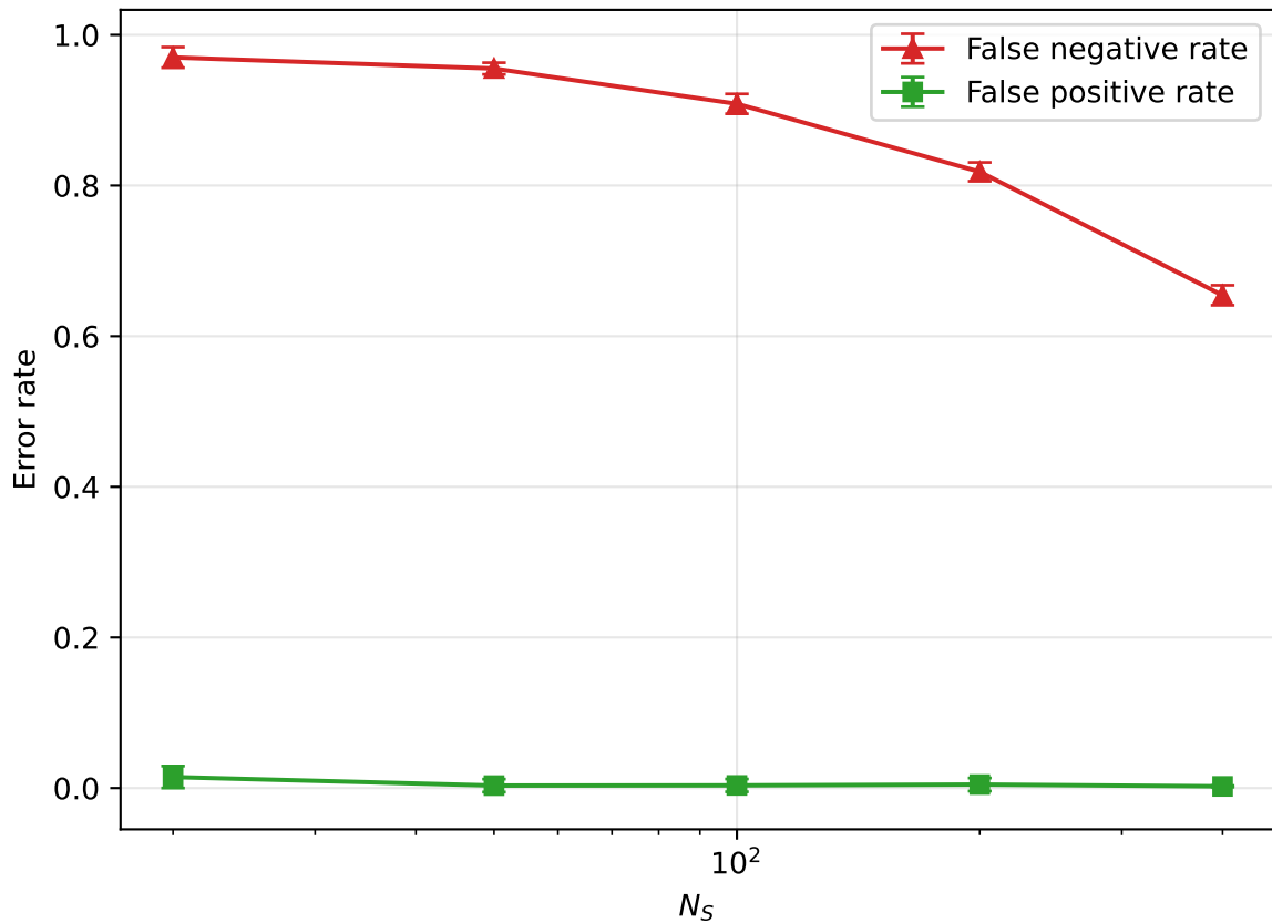
20 Newsgroups (sci.crypt vs sci.electronics): filter errors vs N_S
