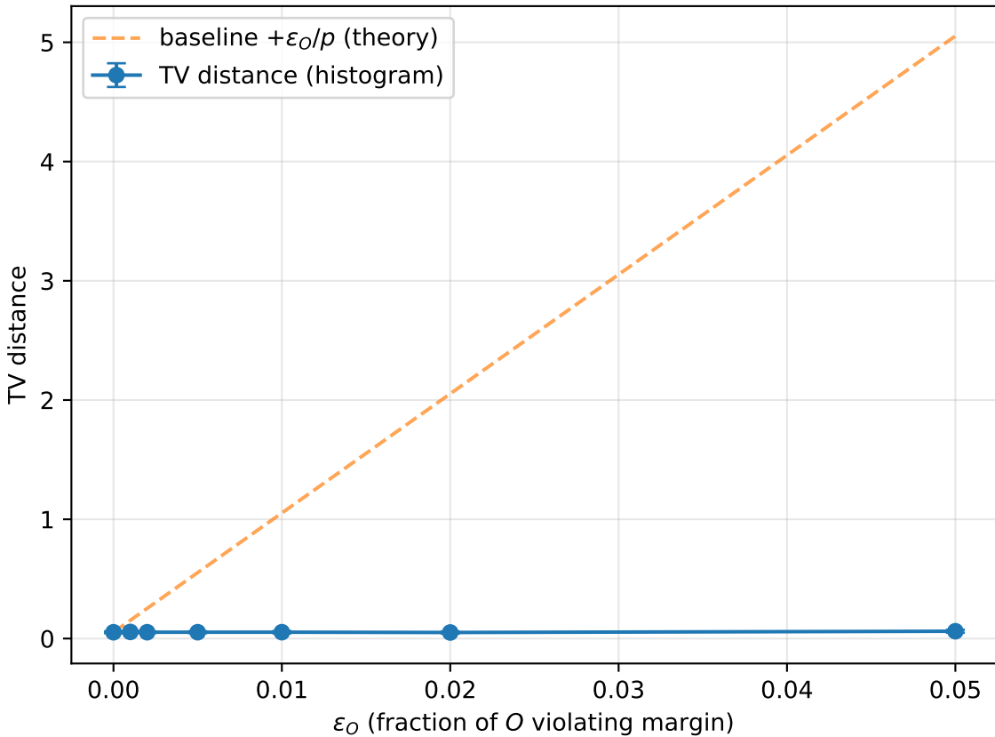
Weak separation: varying \varepsilon_O ( \gamma = 0.1 , d = 50 , N_S = 1000 )
