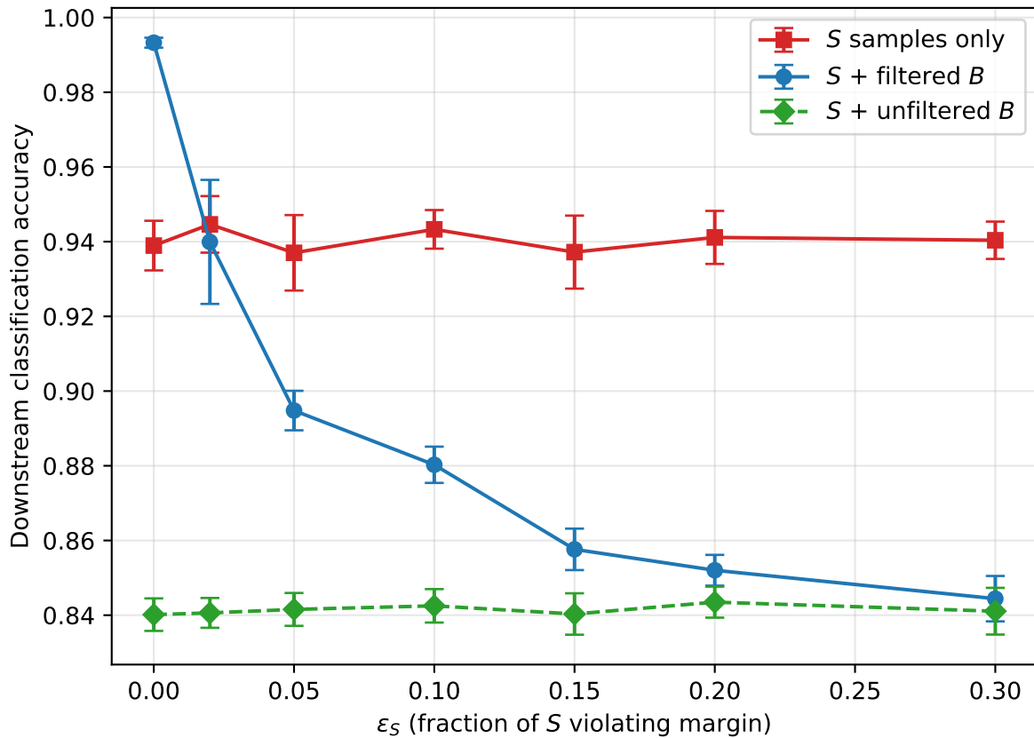
Downstream accuracy vs \varepsilon_S ( \gamma = 0.1 , d = 50 , N_S = 1000 )
