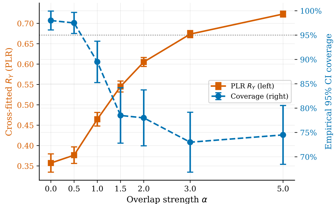
XGBoost, Surface B (Nonlinear)
