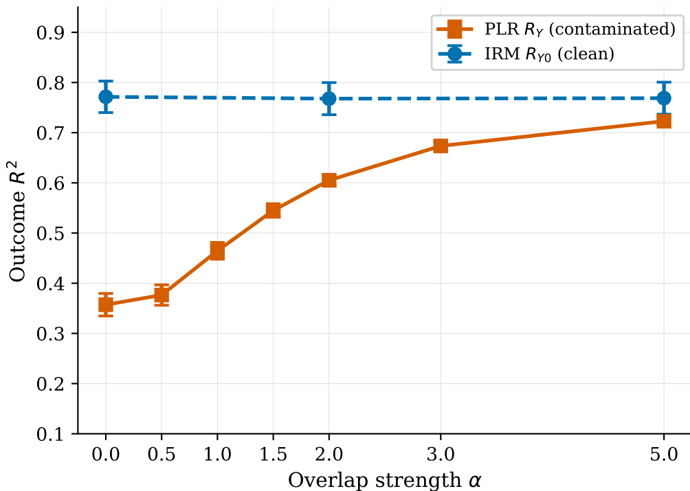
XGBoost, Surface B (Nonlinear)
