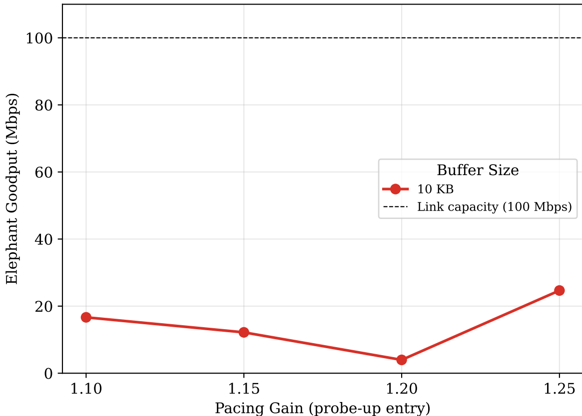
Phase 3: Elephant Goodput vs Pacing Gain (averaged over RTTs)
