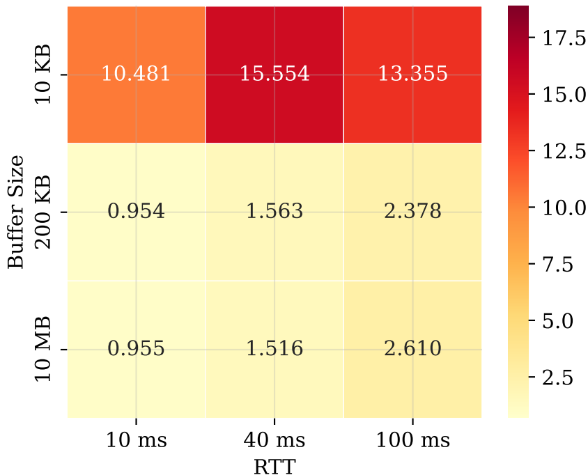
Mean Mice FCT (s) — BBRv1
