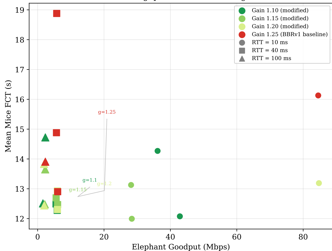
Phase 3: FCT vs Throughput Tradeoff — Pacing Gain Reduction
