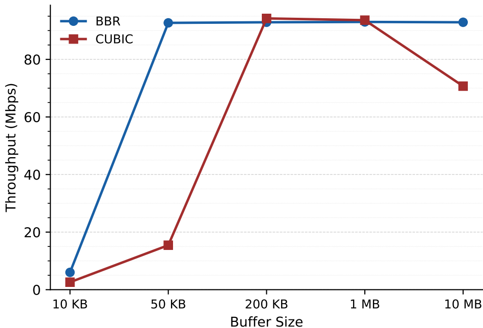
Throughput vs. Buffer Size — BBR vs. CUBIC (Reproducing Cao et al. IMC 2019 §4.1 / Fig. 8a behavior) 100 Mbps link
