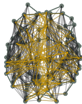
consensus (cost: 340)
