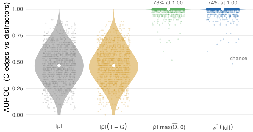
Figure 4: Ablation, estimator-level AUROC (C edges versus distractors) over 1,000 replicates; axis labels give each arm’s scoring formula. Each point is one replicate (horizontal jitter only), violins show the boundary-corrected density, and white dots mark medians. The Gini ablation |\rho|(1 - G) is at chance (mean .464); the coherence-gate ablation |\rho|\max(\bar{O}, 0) carries the effect (.985); the full w^* matches it (.985) — the a-priori prediction of Section 2.3. The right-hand distributions pile at ceiling (73–74% of replicates at AUROC exactly 1.00, annotated), which is why their densities compress into the solid band at the top. The oracle subgroup comparator (mean AUROC .002, inverted) is reported in the text as a diagnostic.
