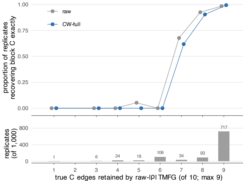
Figure 5: Failure map. Exact-C recovery as a function of the number of true C edges (of ten) retained by the raw- |\rho| TMFG; the structural maximum is nine because K_5 is non-planar. Both pipelines share the same TMFG, so availability is identical by construction; the two methods are dodged horizontally for visibility. The lower panel shows how the 1,000 replicates distribute over availability — each bar is the denominator of the recovery proportion plotted above it, and the distribution is bimodal (nine, or about six when a C item is displaced; retaining exactly two never occurred). Recovery is near-ceiling at maximal availability and collapses below it identically for raw and CW: candidate-edge selection, not the carrier statistic, is the binding constraint.
