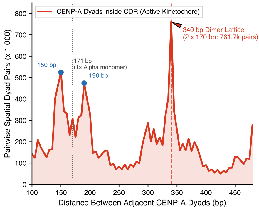
A. CENP-A Spatial Autocorrelation (CDR Phasogram)
