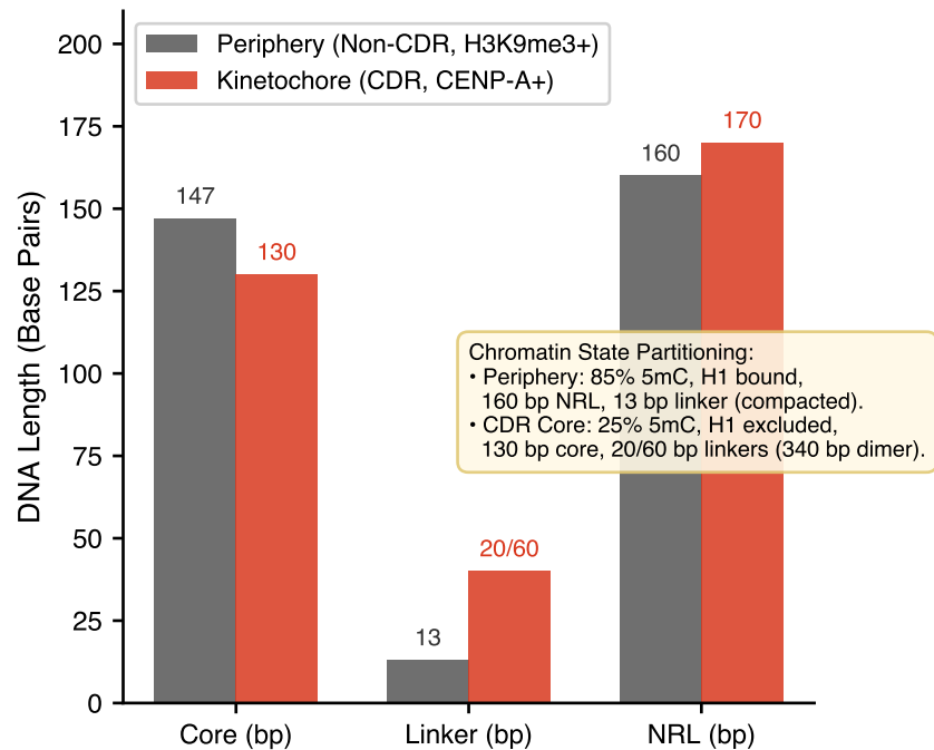
B. Bimodal Centromeric Phase Transition
