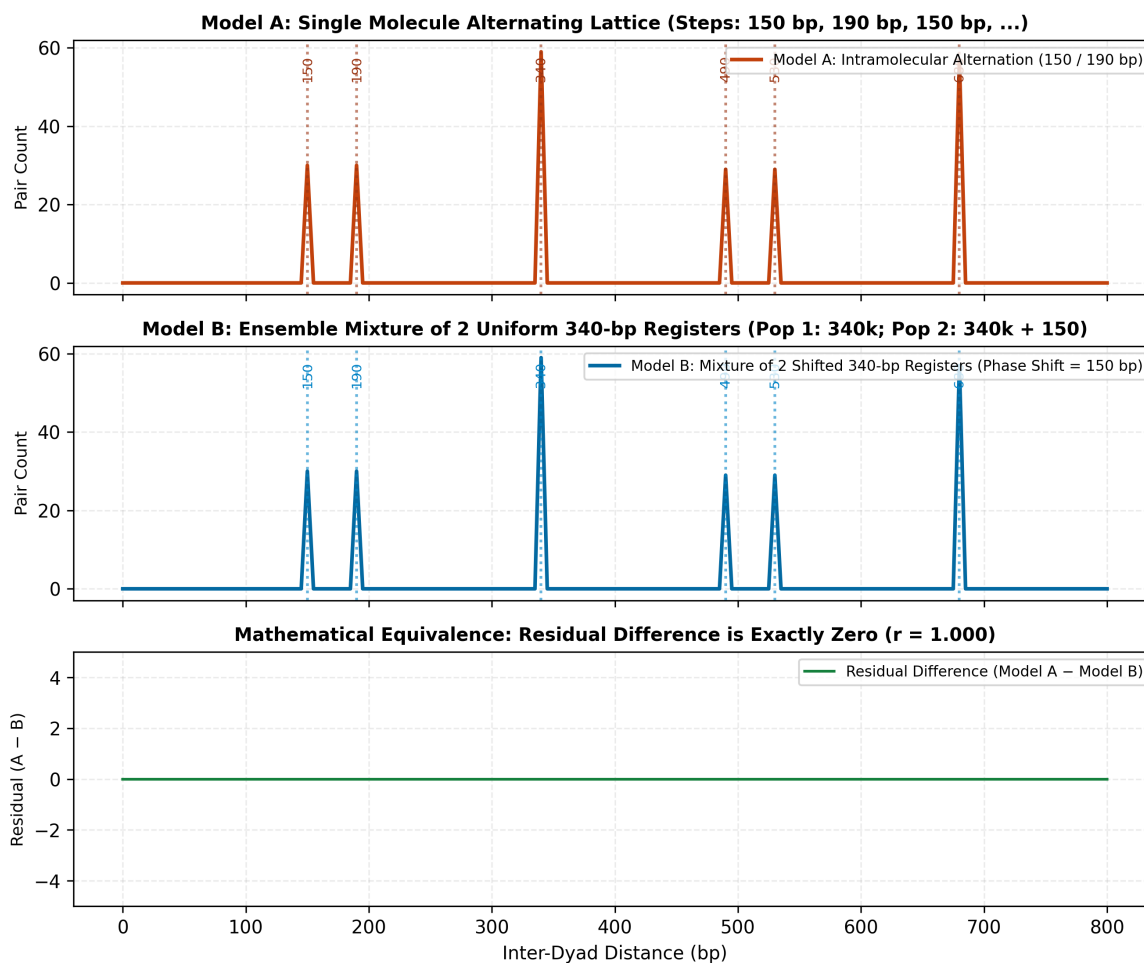
Figure 3: Mathematical Simulation of Alternating vs. Register Mixture Phasing.
