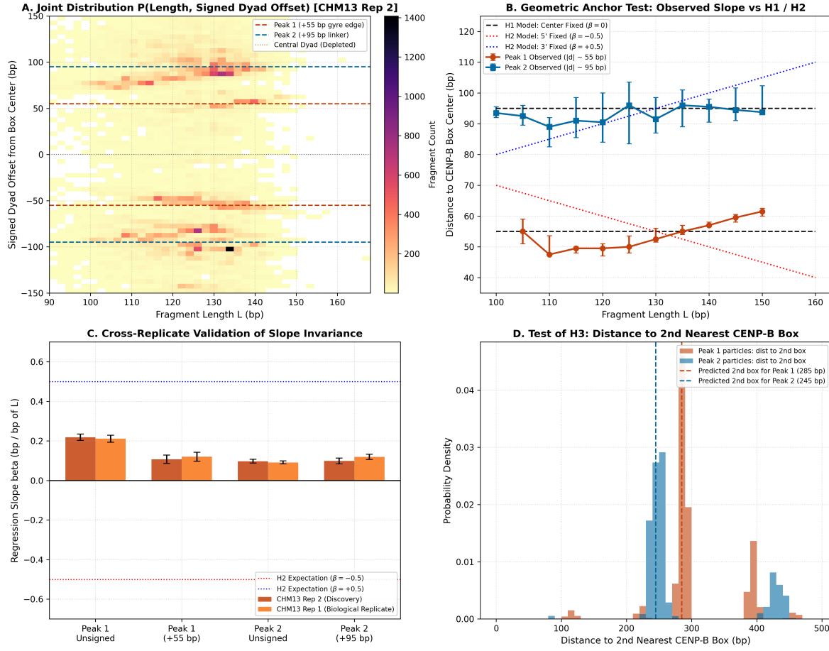
Figure 10: Geometric Anchoring of CENP-B Coupling: Central Dyad vs. Fragment End Dynamics (EXP-03).
