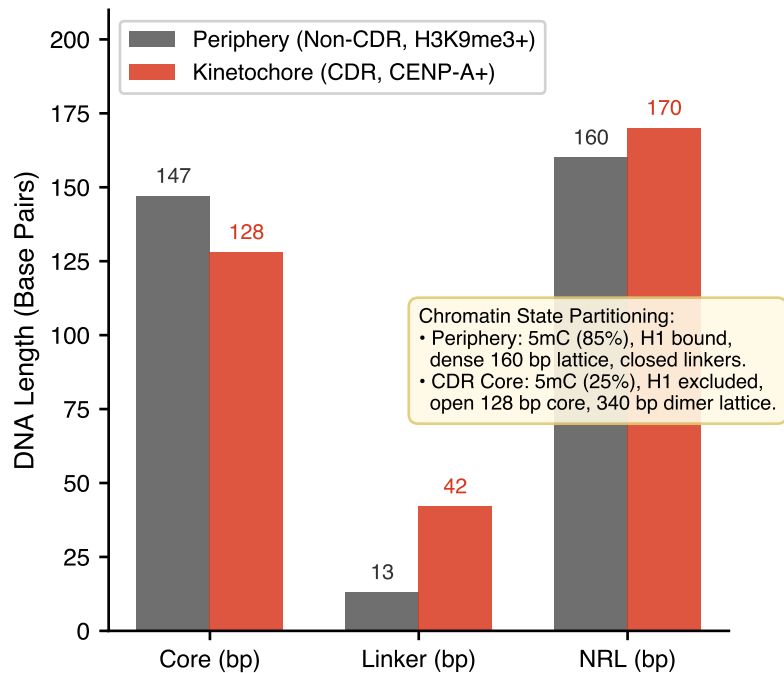
B. Bimodal Centromeric Phase Transition
