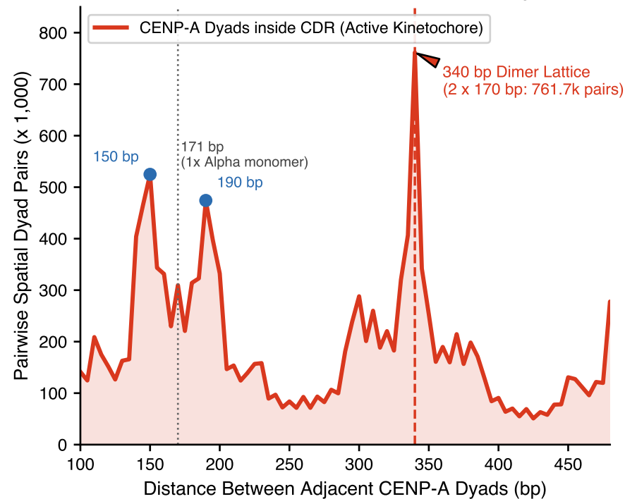
A. CENP-A Spatial Autocorrelation (CDR Phasogram)
