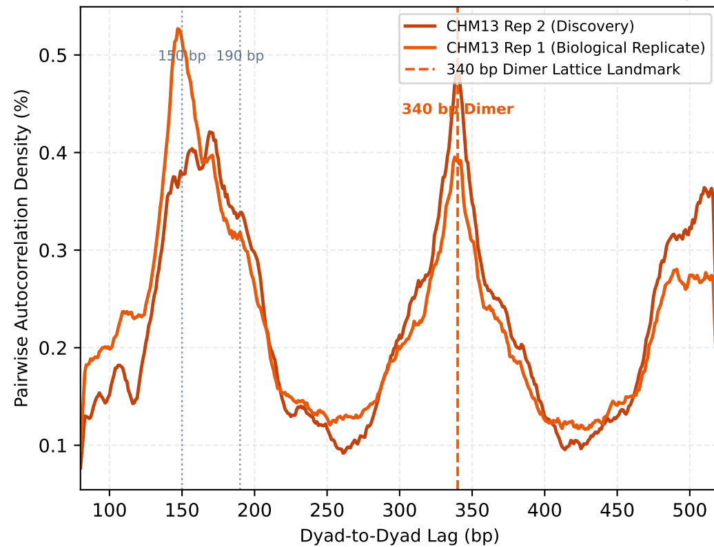
C. Spatial Autocorrelation & 340 bp Dimer Lattice Organization
