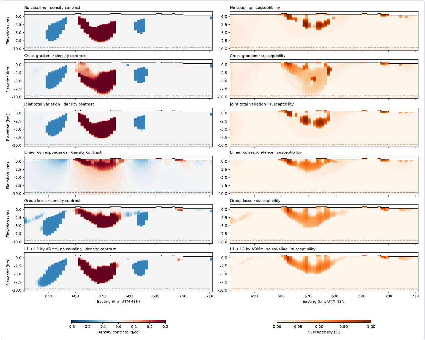
Figure 2 E–W sections through the Sandur belt (northing 1667.5 km): density contrast (left, \pm 0.3 g/cc) and susceptibility (right, square-root scale to 1 SI) for each coupling. The black line is the ground of the mesh, the dashed line the base of the core.
