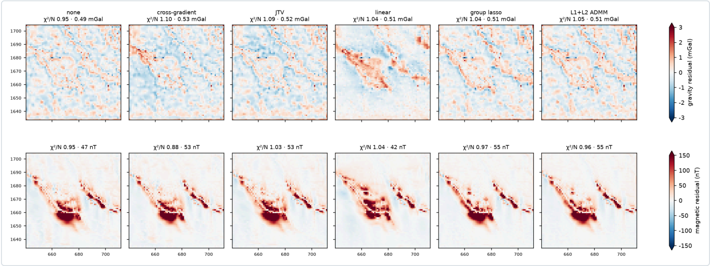
Figure 1 Residuals (observed – predicted) of the gravity data (top, \pm 3 mGal) and the magnetic data (bottom, \pm 150 nT) for each coupling.
