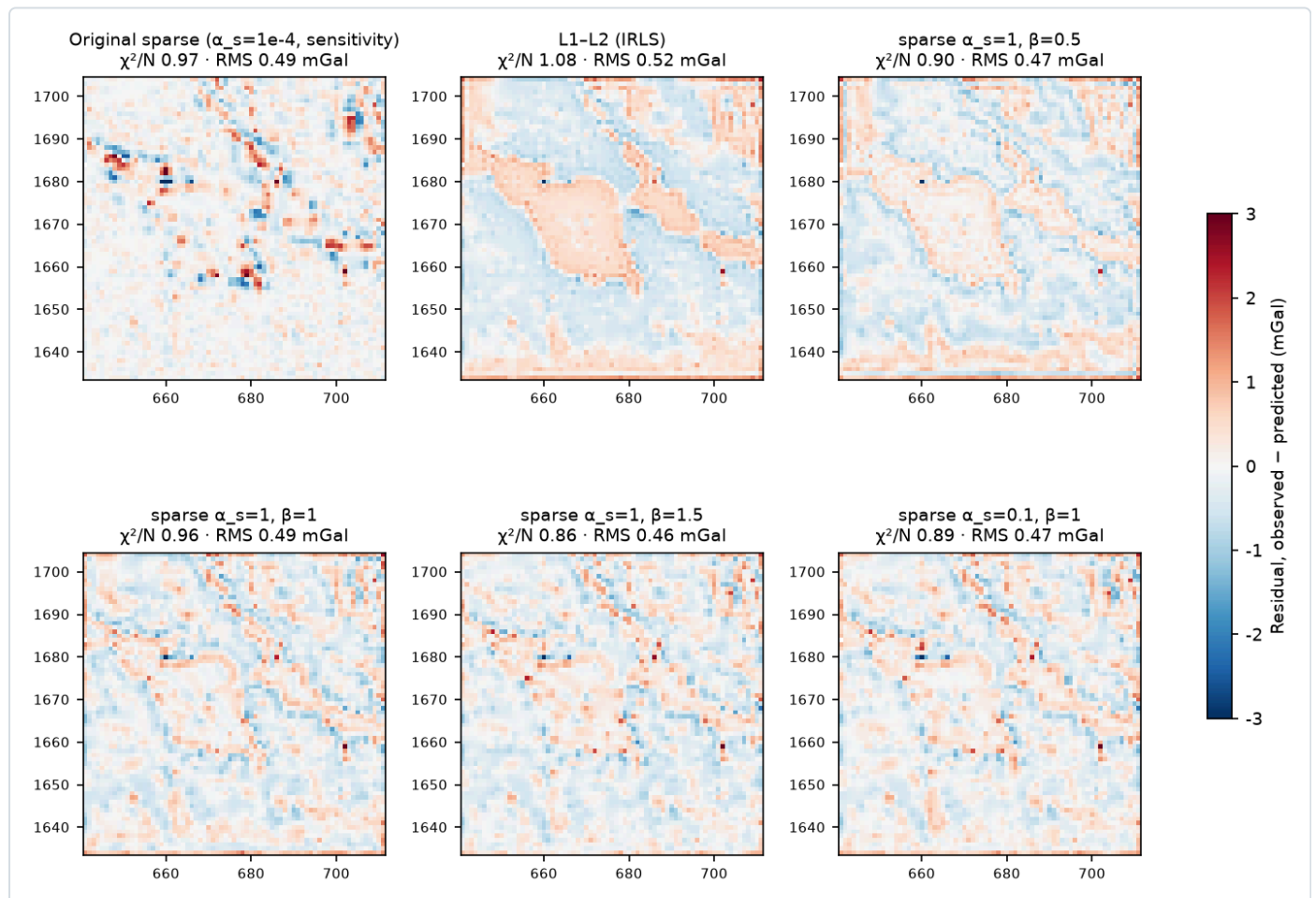
Figure 2 Residuals (observed – predicted) of the six full-resolution models; colour scale \pm 3 mGal.
