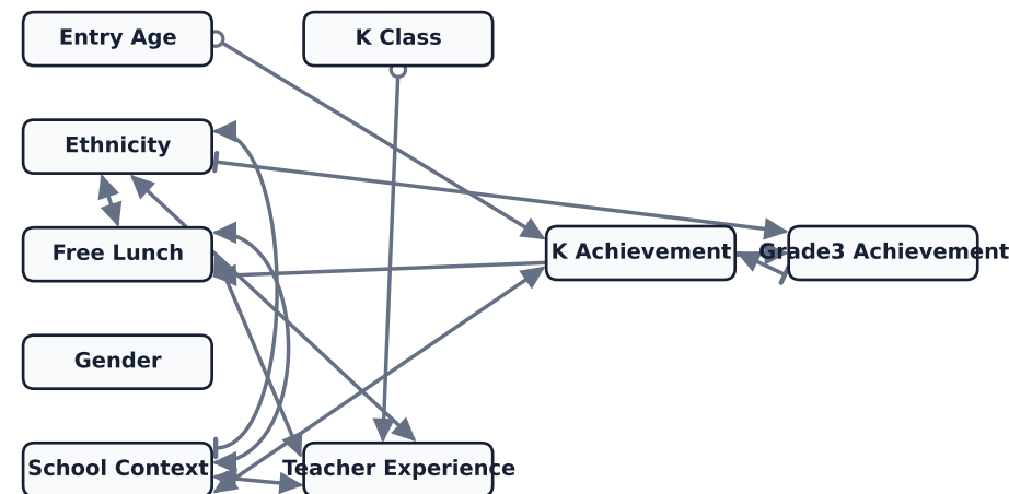
R pcalg::fciPlus 12 edges, 475 CI tests
