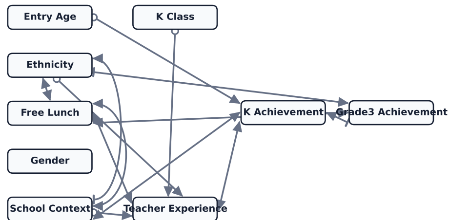
Self-implemented FCI+ 13 edges, 335 CI tests
