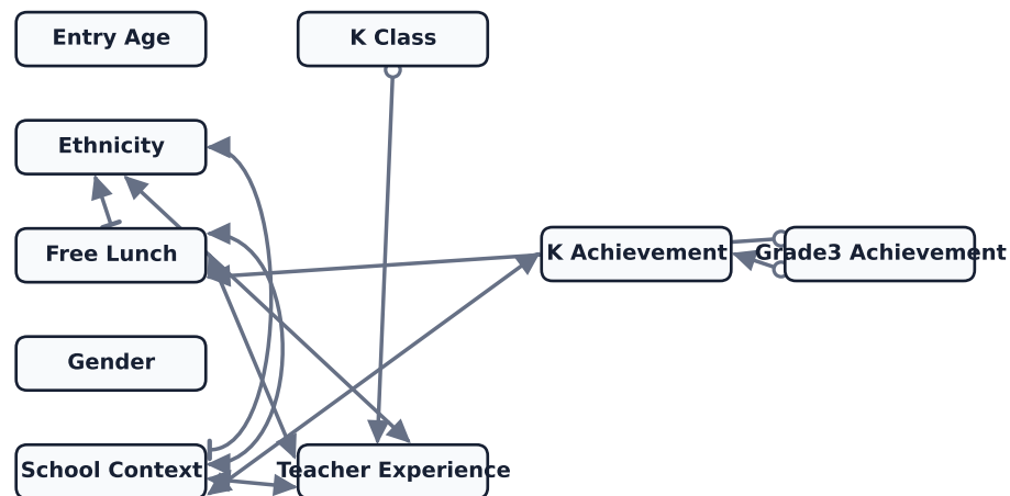
Standard FCI 10 edges, 960 CI tests
