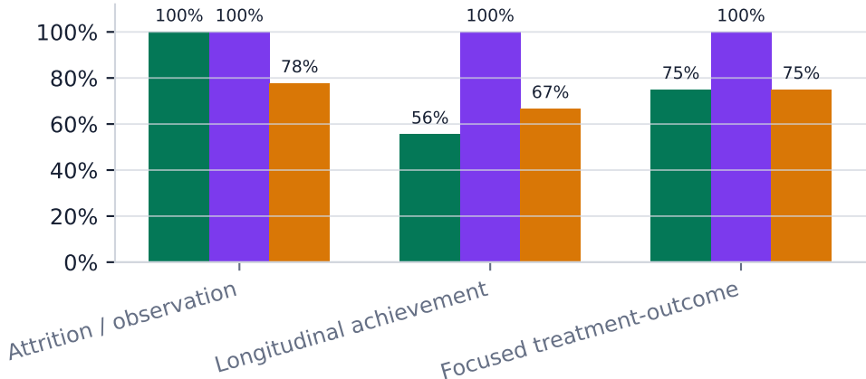
Exact PAG match rate
