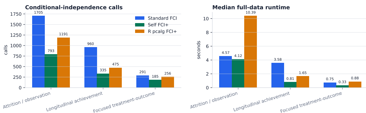
Figure 7.9: Full-data search work and median runtime. All algorithms use the same panel, compact-table G-square test, and \alpha = 0.05 ; internal search schedules and language runtimes are not identical.
