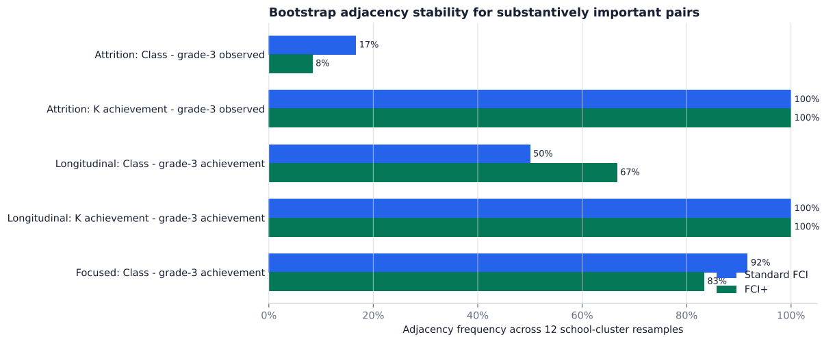
Figure 7.5: School-cluster adjacency frequencies for selected pairs. Frequencies measure skeleton stability only; they do not validate endpoint orientation.
