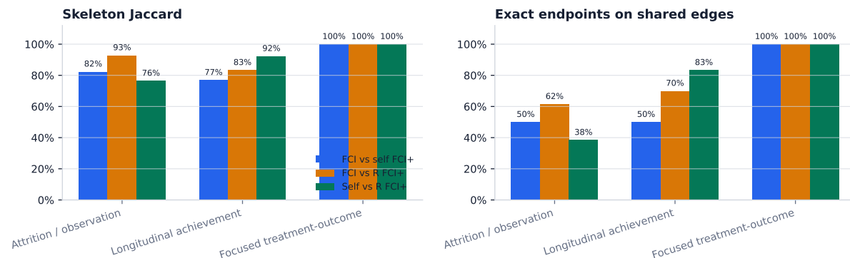
Figure 7.7: Pairwise skeleton Jaccard and exact endpoint agreement on shared edges. Skeleton agreement is consistently stronger than endpoint agreement outside the focused panel.
