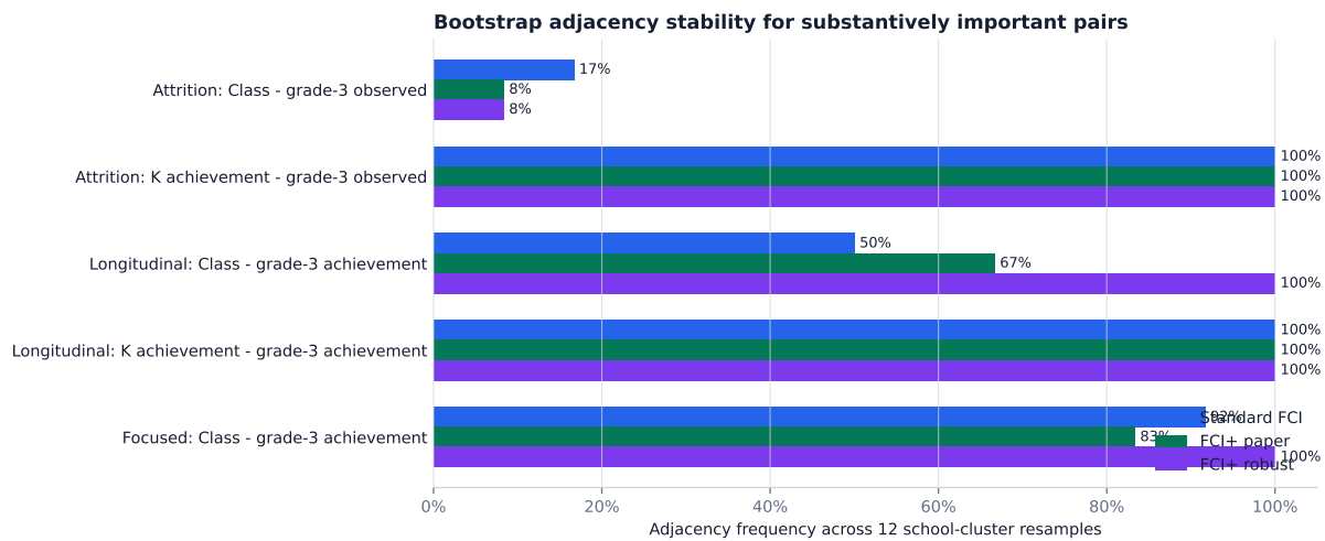
Figure 10.6: School-cluster adjacency frequencies for selected pairs. Frequencies measure skeleton stability only; they do not validate endpoint orientation.
