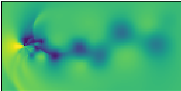
Ground truth
