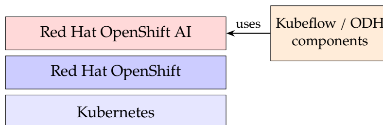
Figure 3.1: The platform stack: Kubernetes provides container orchestration, OpenShift adds enterprise features, and Red Hat OpenShift AI is the commercial ML platform that uses Kubeflow and Open Data Hub components (such as the Notebook Controller).
