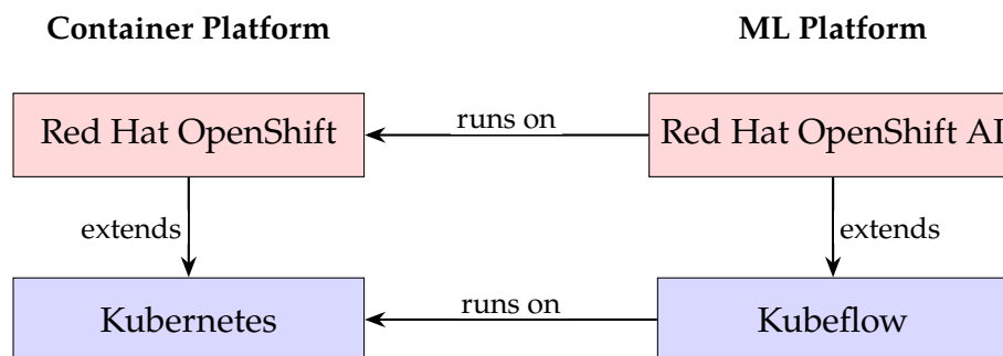
Figure 3.1: The platform stacks showing the relationships between open-source projects and their enterprise counterparts. Vertical arrows show how Red Hat extends the upstream projects with enterprise features. Horizontal arrows show runtime dependencies: Kubeflow runs on Kubernetes, and RHOAI runs on OpenShift. RHOAI incorporates Kubeflow components via the Open Data Hub community project.
