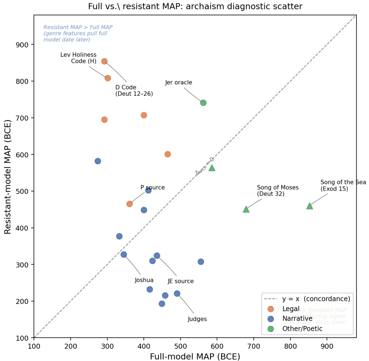
Fig 4. Full versus resistant MAP dates: archaism diagnostic scatter plot. Each of 22 analyzed textual units is plotted with full-model MAP ( x -axis) versus resistant-model MAP ( y -axis); filled circles = non-noisy texts, triangles = short or noisy texts. Colour indicates genre: blue = narrative, orange = legal, green = other/poetic. The diagonal dashed line indicates concordance ( \Delta_{\text{arch}} = 0 ). Points below the diagonal (full MAP > resistant MAP, \Delta_{\text{arch}} > 0 ) signal archaizing composition—the full model dates the text more ancient than its clause-level syntax alone would suggest. Points above the diagonal ( \Delta_{\text{arch}} < 0 ) indicate that genre features systematically pull the full-model date later than the underlying resistant syntax. Song of the Sea (Exod 15; \Delta_{\text{arch}} = +392 yr) and D_Code (Deut 12-26; \Delta_{\text{arch}} = -562 yr) are the most extreme positive and negative outliers, respectively.
