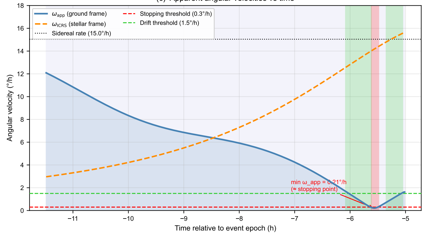
(c) Apparent angular velocities vs time
