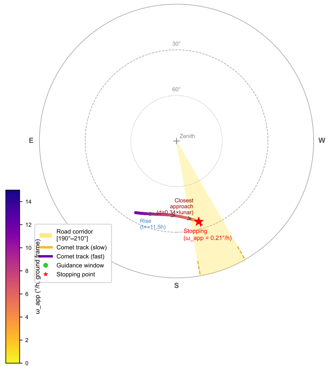
(a) Sky track: Bethlehem, 5 BCE Best close-flyby orbit — N up, E left
