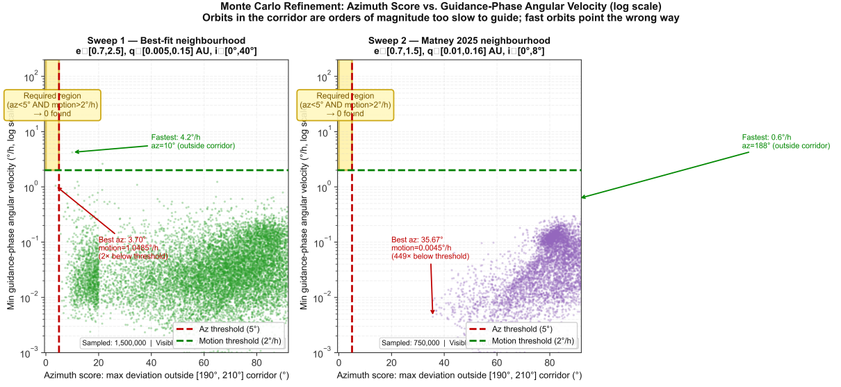
Figure S1: Supplementary Figure S1: Monte Carlo refinement sweeps — azimuth score vs. guidance-phase angular velocity (log scale). Each point is one visible orbital configuration from the two continuous-parameter sweeps described in §S1.7. Left (Sweep 1): 1.5 million configurations in the neighborhood of the best-fit grid orbit ( e \in [0.7, 2.5] , q \in [0.005, 0.15] AU, i \in [0^\circ, 40^\circ] , all \Omega/\omega , \Delta T \in [-60, +60] days); 601,150 visible, 0 satisfying all criteria. Right (Sweep 2): 750,000 configurations in the neighborhood of Matney’s (2025) proposed 5 BCE comet ( e \in [0.7, 1.5] , q \in [0.01, 0.16] AU, i \in [0^\circ, 8^\circ] , \Omega \in [26^\circ, 126^\circ] , \omega \in [286^\circ, 386^\circ] ); 294,672 visible, 0 satisfying all criteria. In both panels the gold shaded region marks the zone where both the azimuth criterion ( < 5^\circ ) and guidance-motion criterion ( > 2^\circ h^{-1} ) are simultaneously satisfied. The log scale reveals the structural anti-correlation: objects in the road corridor are orders of magnitude too slow to guide ( \sim 0.006^\circ h^{-1} , a factor of \sim 330 below threshold in Sweep 1), while the fastest objects point in entirely the wrong direction.
