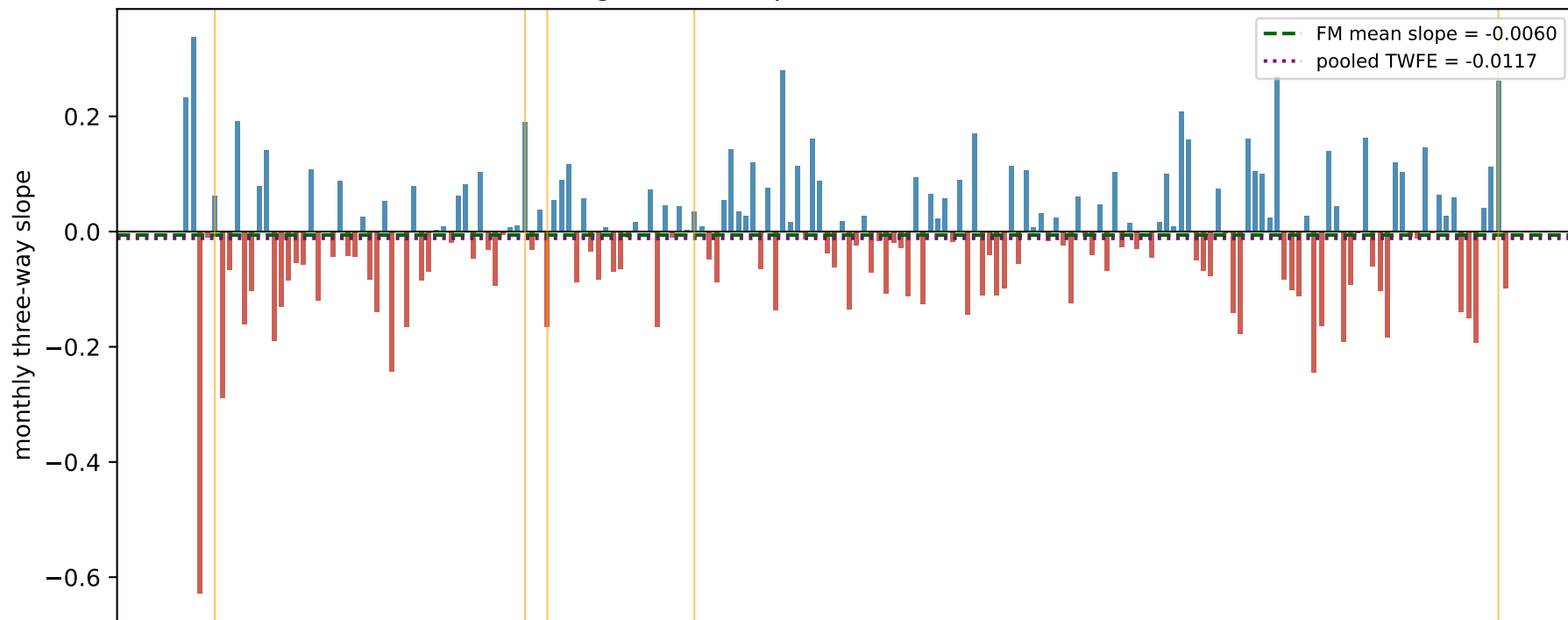
Monthly cross-sectional three-way slopes (FM coefficients), 2009-2023 (orange lines = top-5 TWFE-influence months)
