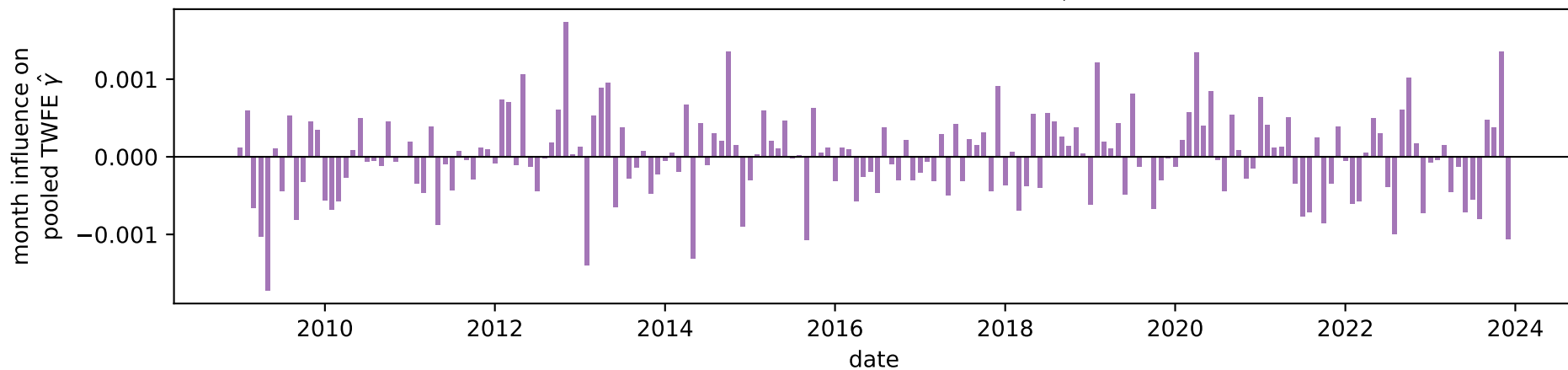
Jackknife-by-month influence: \hat{\gamma}_{full} - \hat{\gamma}_{drop\ month}
