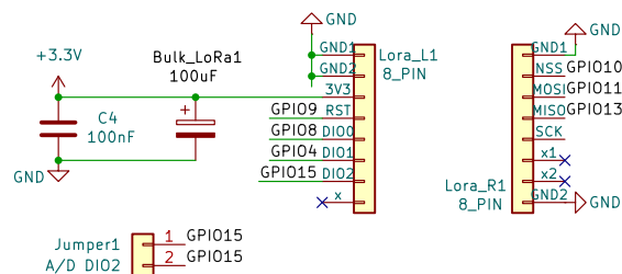
Circuit_Lora
