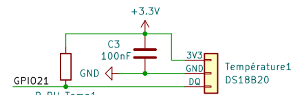
Circuit_1Wire
