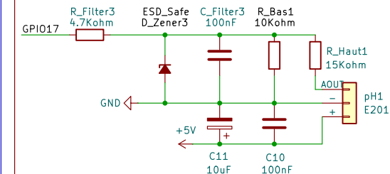
Circuit_pH
