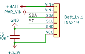
Circuit_PowerControl
