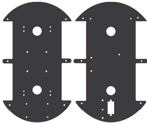
Bottom Plate*1PC
